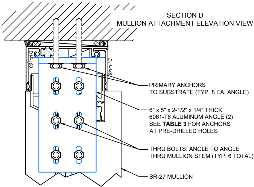
MULLION ATTACHMENT AT HEAD (SEE SHEETS 1, 2, 4, & 5 FOR ANCHORAGE DETAILS AT ALL OTHER LOCATIONS)
