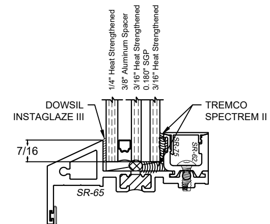
E MISSILE GLAZING DETAIL
