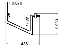
INSERT, SLOPE - FX/AWN & FX/CASEMENT SR-64
