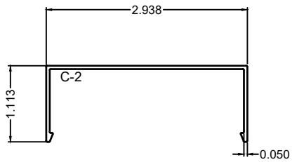
COVER, MULLION CLAMP C-2
